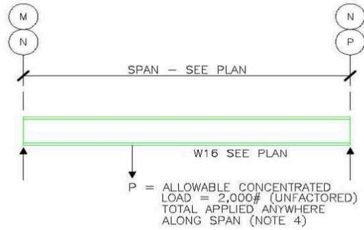
THEATRE AREA PURLIN
